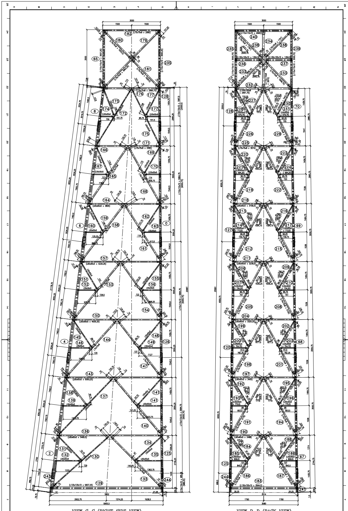
VIEW C-C (RIGHT SIDE VIEW)
